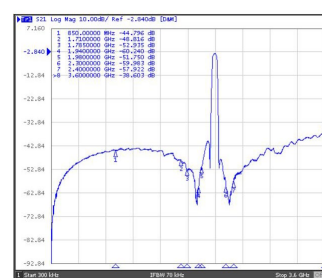
Figure 2. Electrical Characteristics: Wideband
