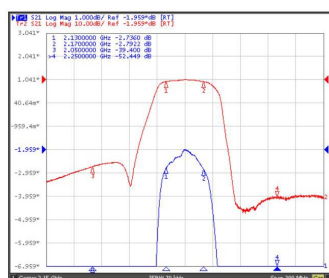
Figure 1. Electrical Characteristics: Frequency response
