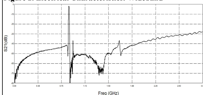
Figure 2. Electrical Characteristics: Wideband
