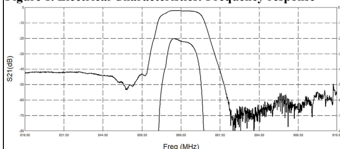
Figure 1. Electrical Characteristics: Frequency response
