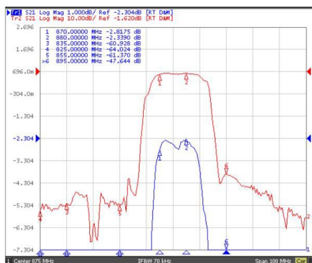
Figure 1. Electrical Characteristics: Frequency response
