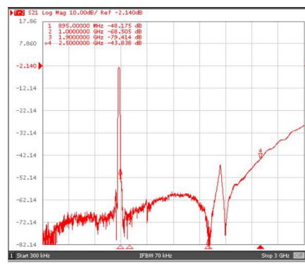
Figure 2. Electrical Characteristics: Narrowband
