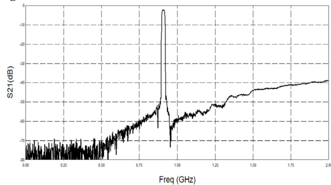
Figure 2. Electrical Characteristics: Wideband
