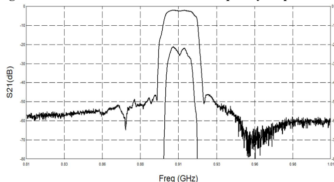
Figure 1. Electrical Characteristics: Frequency response
