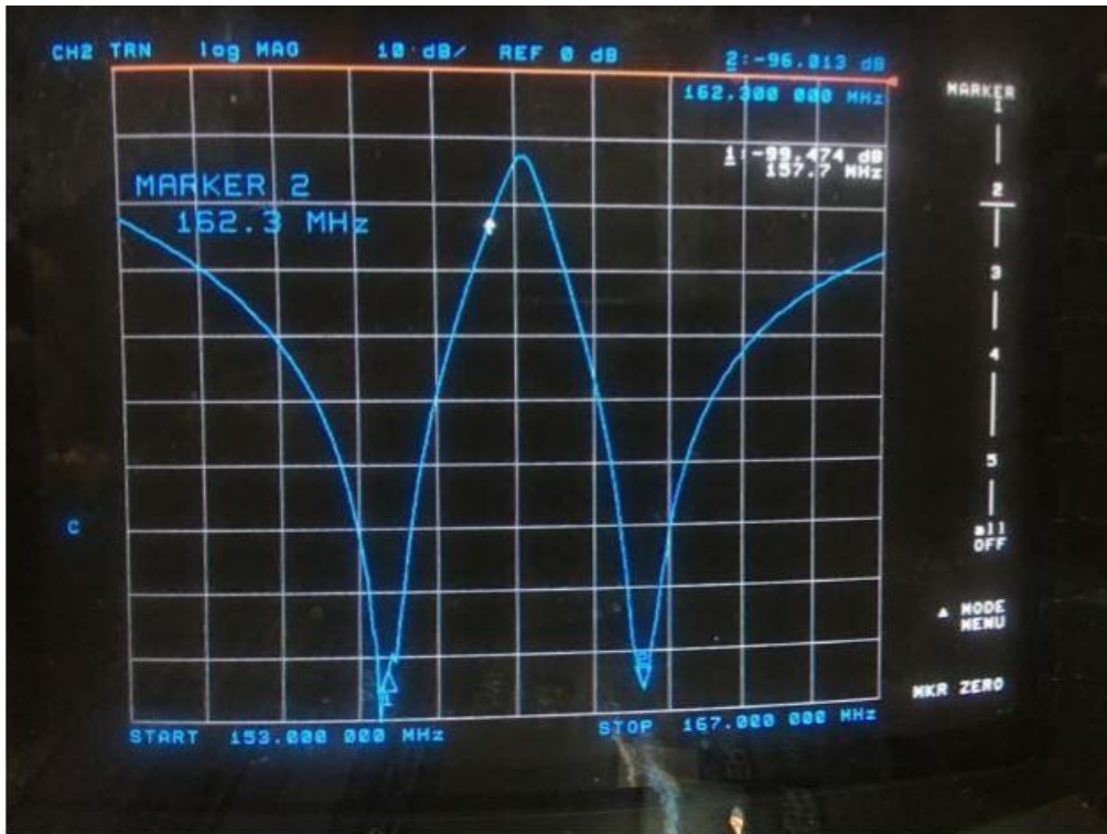
157.700MHz Isolation: -99.47, 162.300MHz Isolation: -96.01
