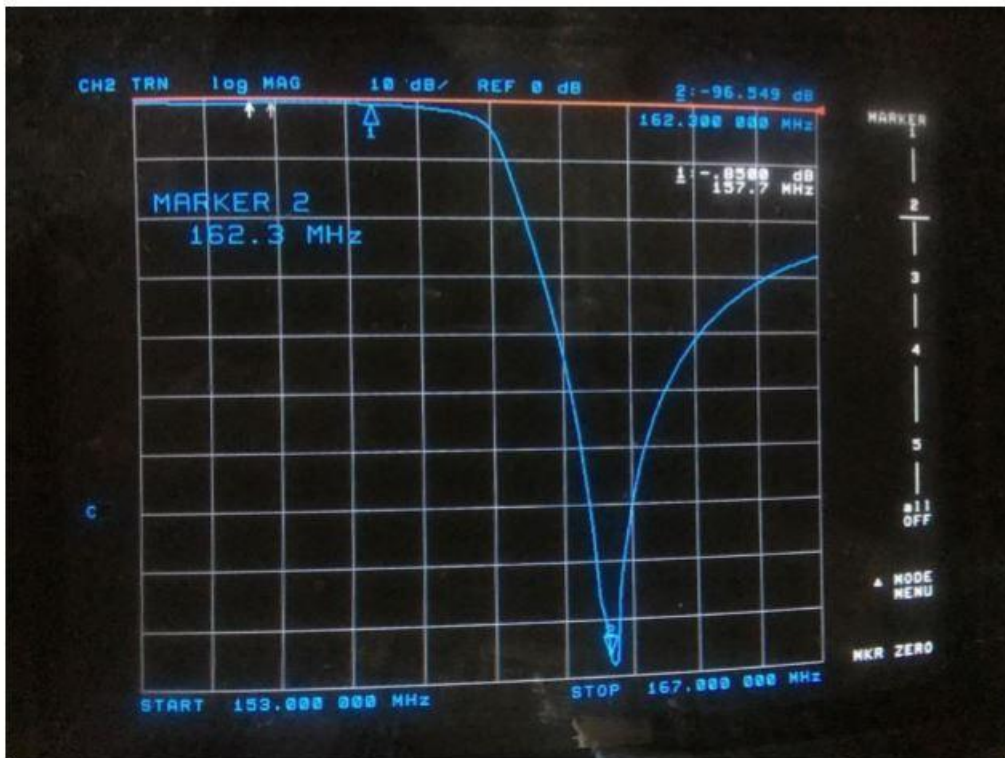
157.700MHz Insertion Loss: 0.85
