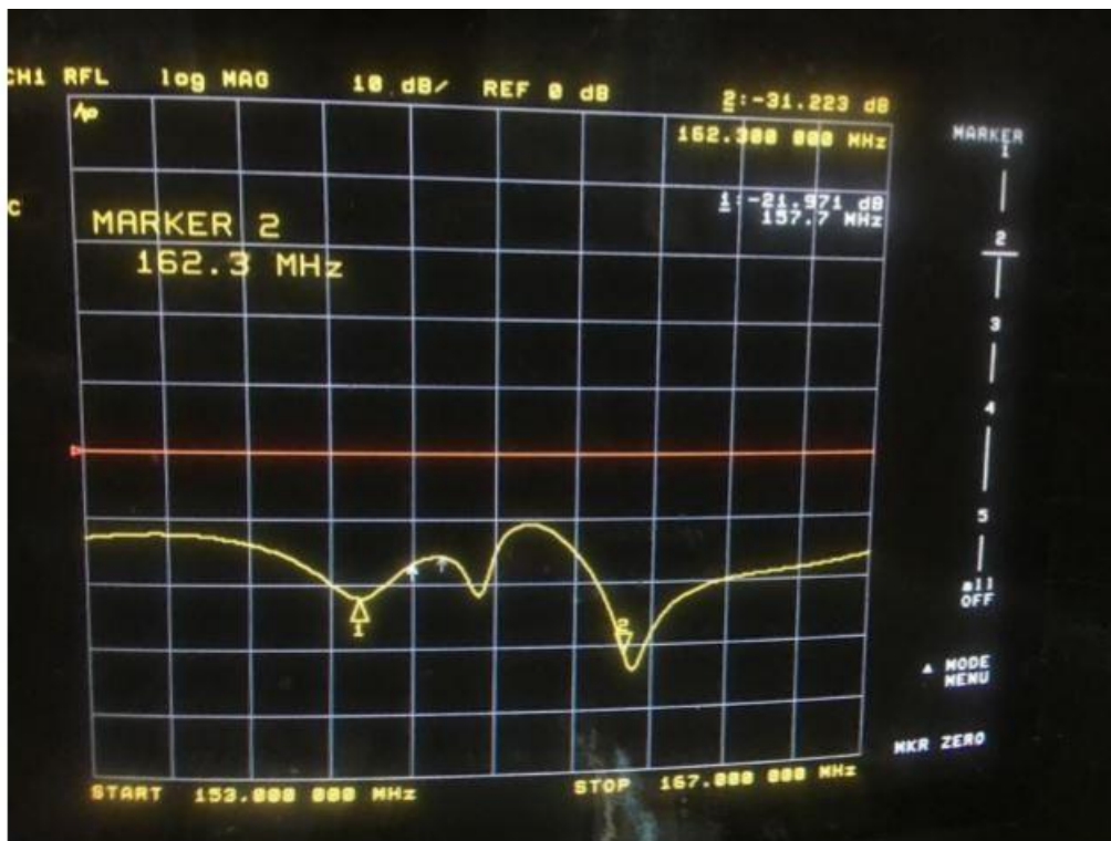
157.700MHz Return Loss: 21.971, 162.300MHz Return Loss: 31.223
