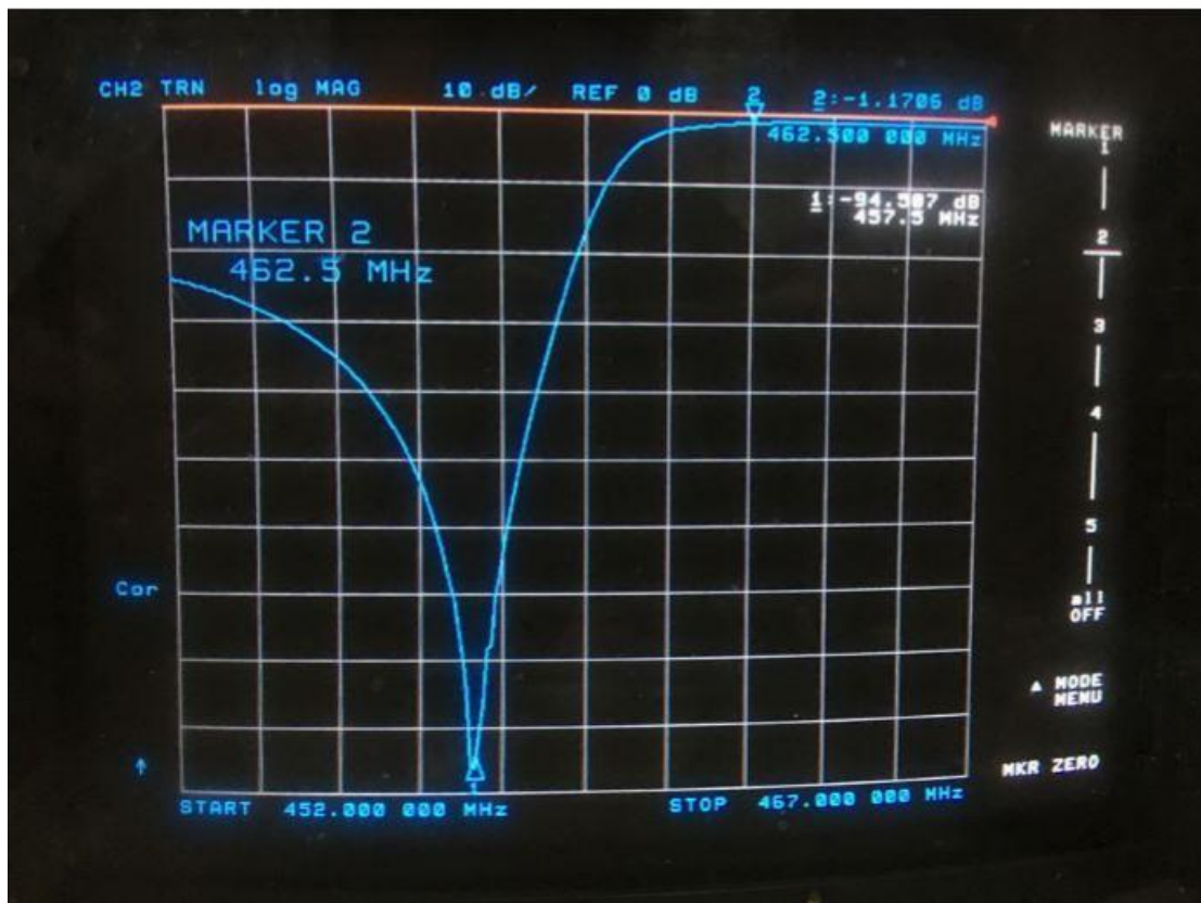
462.500MHz Insertion Loss:1.170
