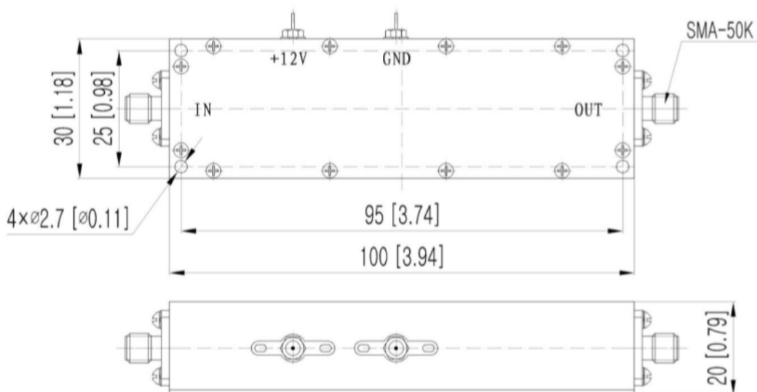
Outline drawing (unit: mm )
